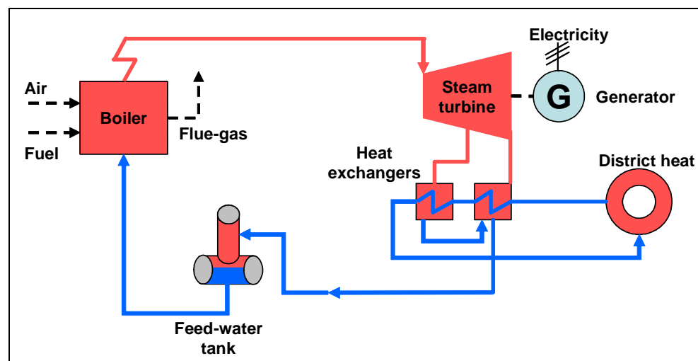
Figure 3.12: Backpressure plant [65, Nuutila, 2005]
