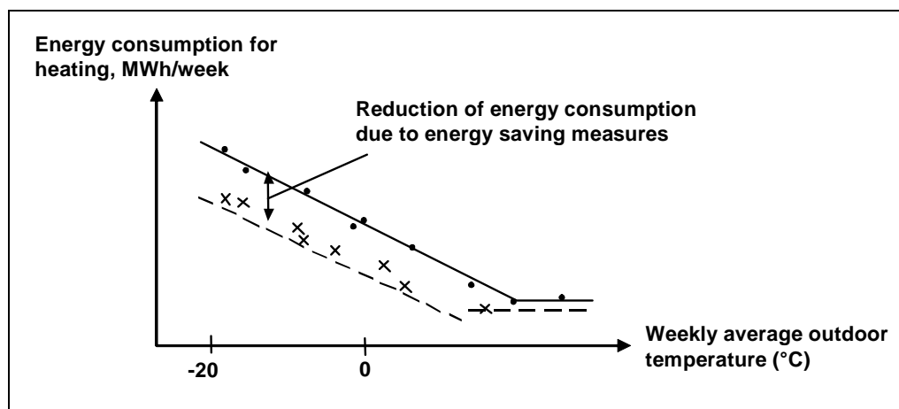
Figure 1.17: Energy consumption depending on outdoor temperature
